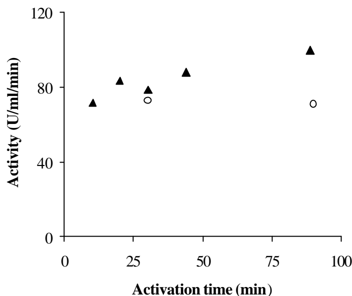
Figure 4.5 Effects of activation on the activities of sulfhydrogenase. (σ) H 2 -uptake (measured at 60 °C). (o) H 2 evolution (measured at 80 °C).
