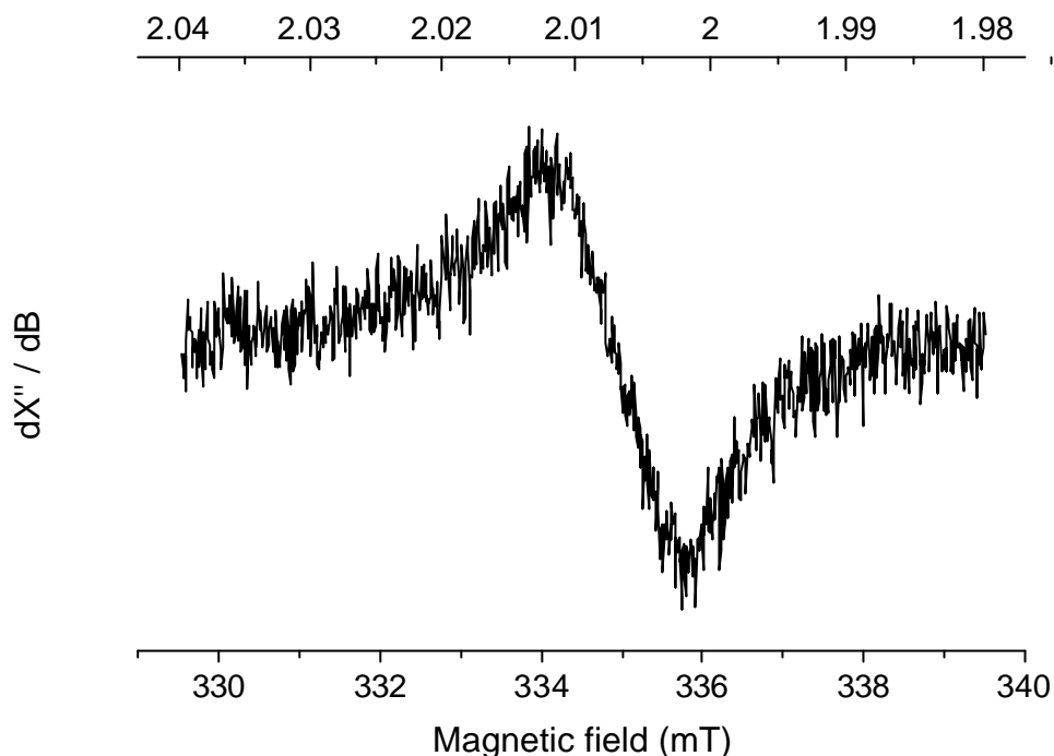
Figure 4.6 EPR spectrum of the flavin radical present in sulfhydrogenase. EPR conditions: microwave frequency, 9.4078 GHz; microwave power, 0.2 \mu W ; temperature, 16.5 K.
