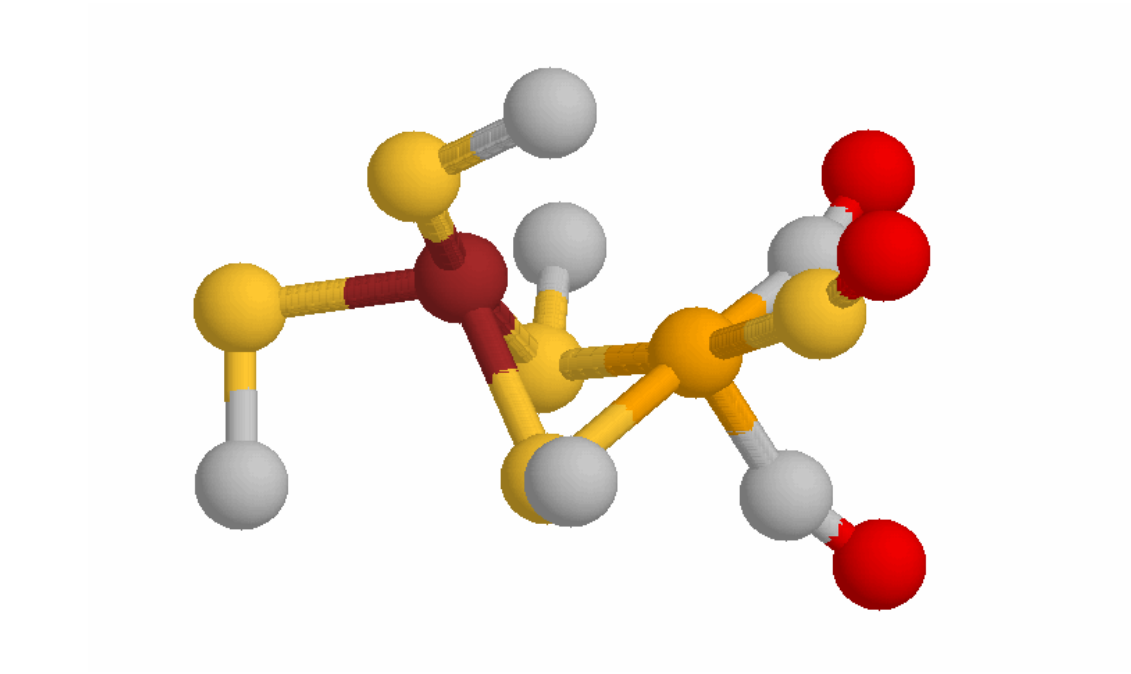
Figure 2.4 X-Ray crystal structure (at 1.8 Å resolution) of the reduced NiFe hydrogenase from D. vulgaris Miyazaki F (Higuchi et al. , 1999b). Nickel: brown; Iron: orange; Sulfur: yellow; Carbon: grey; Oxygen: red.
