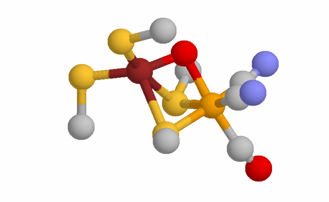
Figure 2.3 X-Ray crystal structure (at 2.45 Å resolution) of the oxidized periplasmic NiFe hydrogenase from D. gigas (Volbeda et al. , 1996). Nickel: brown; Iron: orange; Sulfur: yellow; Carbon: grey; Oxygen: red; Nitrogen: blue.
