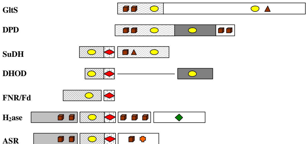
Figure 5.6 A graphical comparison of prosthetic-group binding motifs suggestively identifies P. furiosus sulfide dehydrogenase, SuDH, as a member of two different flavo-iron-sulfur protein 'superfamilies'. Suda is a paradigm for the GltS small subunit-like proteins (in wavy pattern), and SudB is a paradigm for the 'plant-type' reductase + ferredoxin like proteins (in diagonal stripes + vertical dash). Prosthetic groups are presented by symbols: brown cubes for [4Fe-4S], brown triangles for [3Fe-4S], red diamonds for [2Fe-2S], yellow ellipses for FAD/FMN, a dark green diamond for the Ni-Fe dimer in hydrogenase, and an orange cross for the siroheme in sulfite reductase. GltS, glutamate synthase ( Azospirillum brasilense ); DPD, dihydropyrimidine dehydrogenase (porcine liver); SuDH, sulfide dehydrogenase ( P. furiosus ); DHOD, dihydroorotate dehydrogenase ( Lactococcus lactis ); FNR, ferredoxin: NADP + oxidoreductase (Spinach); Fd, ferredoxin (Spinach); H 2 ase, sulfhydrogenase ( P. furiosus ); ASR, assimilatory sulfite reductase ( Salmonella typhimurium ).
