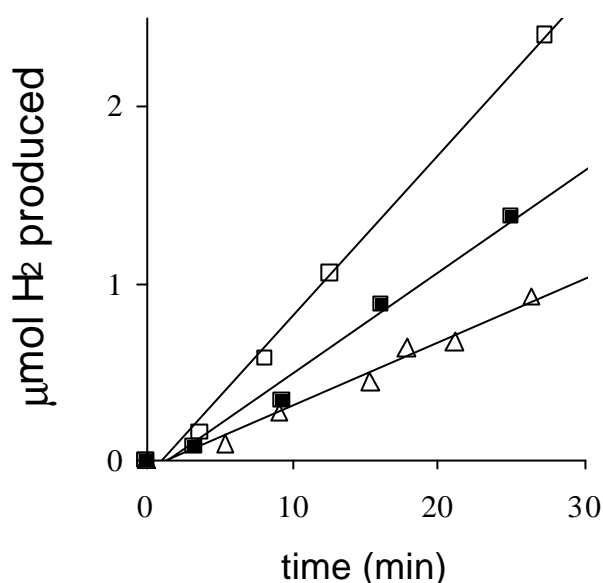
Figure 6.9 H 2 evolution from ferredoxin-reduced Mbh-core complex. (Δ) 7 nmol Fd; (■) 10 nmol FD; (□) 20 nmol Fd. Ferredoxin was reduced in situ by the POR system ( 10 mM pyruvate, 1 mM MgCl 2 , 0.9 mM CoASH, 0.9 mM dithiothreitol, 60 μg POR), and H 2 evolution was measured by gas chromatography. The purified hydrogenase complex was 170 μg protein/ml.
